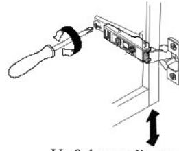
Up&dowr adjustment
