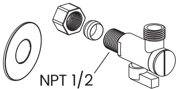
Angle Valve
