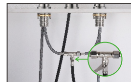
3.Connect the pull down hose and the short hot and cold water supply hoses to the T-connector. Use the provided small wrench to tighten all connections to prevent leaks.
